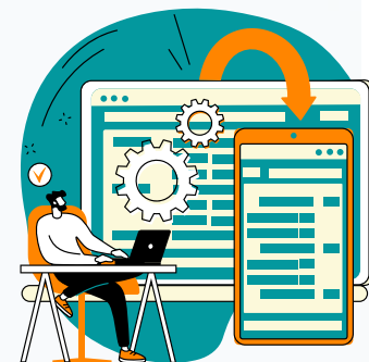
App developers
