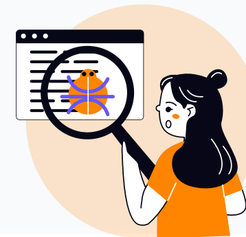
Quality Assurance
