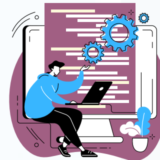
Back-End Developers
