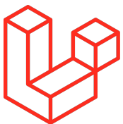
Laravel
