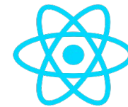
React
