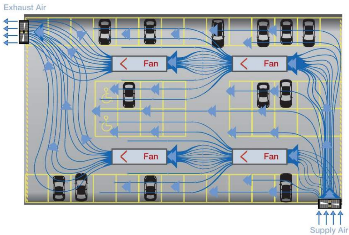
Ventilation System
