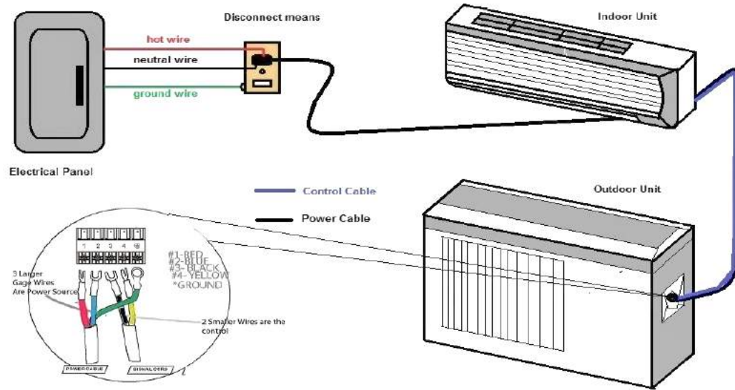
Split Type Air Conditioning System
