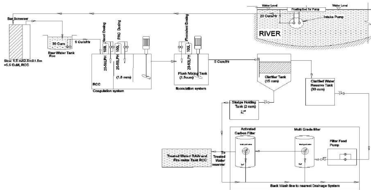
Block Diagram: Schematic Diagram for Water Treatment Plant With Accessories.
